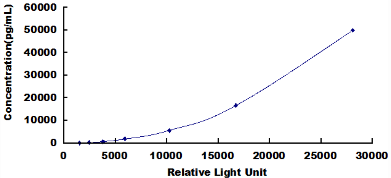
Typical Standard Curve for b2M, Human CLIA.
